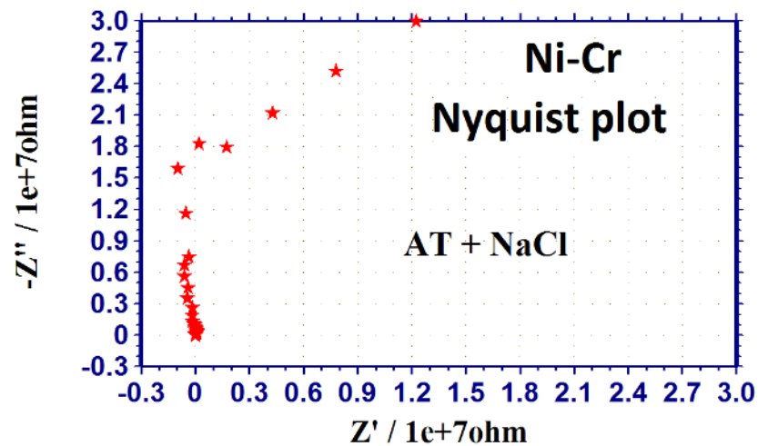
Figure 12. AC impedance spectrum of Ni–Cr immersed in artificial tears + NaCl (Nyquist plot).
