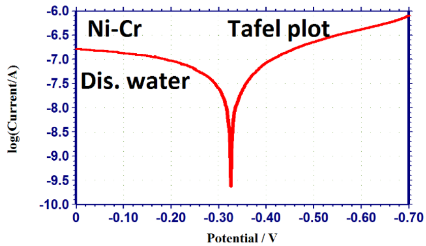
Figure 1. Polarisation curve of Ni–Cr alloy immersed in distilled water.
