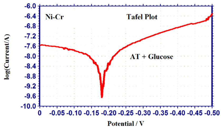
Figure 3. Polarisation curve of Ni–Cr alloy immersed in Artificial Tear + Glucose 500 ppm.
