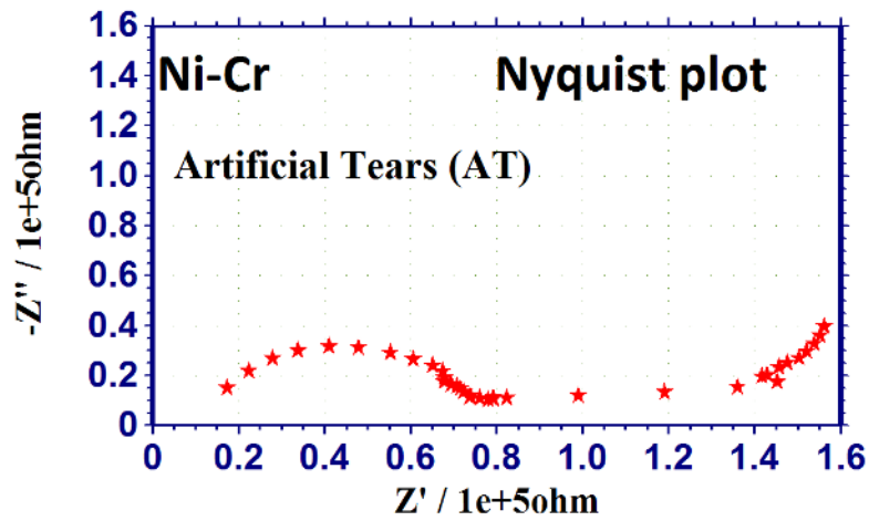
Figure 8. AC impedance spectrum of Ni–Cr immersed in artificial tears (Nyquist plot).
