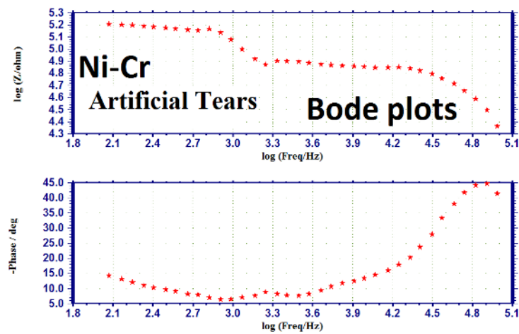
Figure 9. AC impedance spectrum of Ni–Cr immersed in artificial tears (Bode plot).
