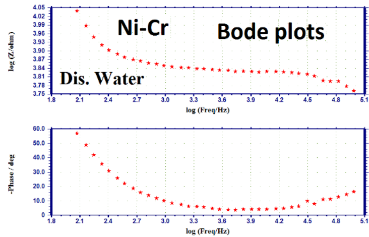
Figure 7. AC impedance spectrum of Ni–Cr immersed in distilled water (Bode plot).
