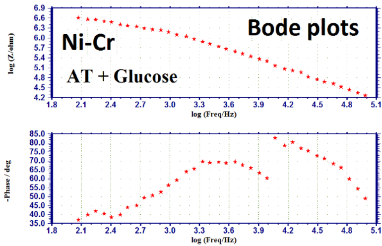
Figure 11. AC impedance spectrum of Ni–Cr immersed in artificial tears + glucose (Bode plot).
