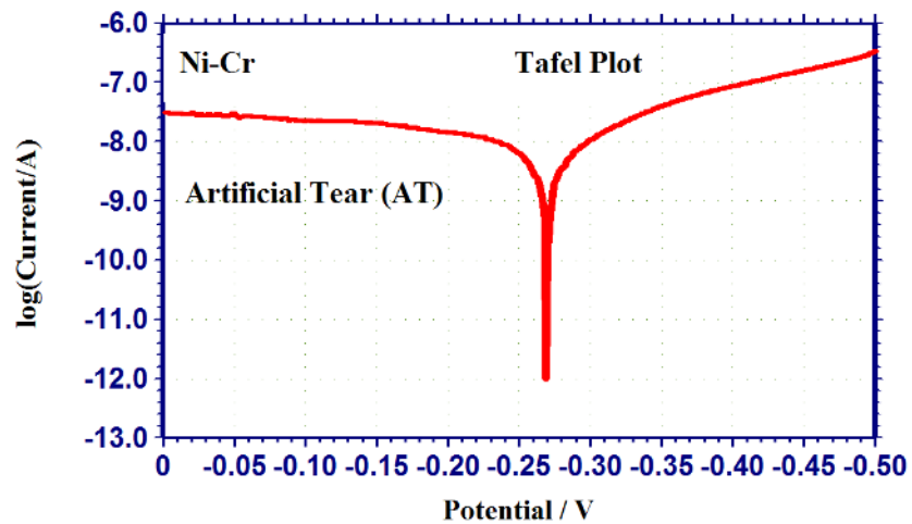
Figure 2. Polarisation curve of Ni–Cr alloy immersed in Artificial Tears.
