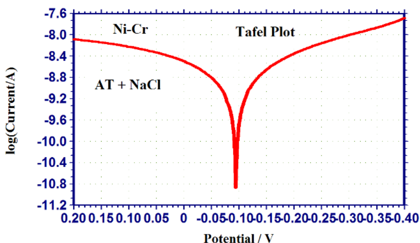
Figure 4. Polarisation curve of Ni–Cr alloy immersed in Artificial Tear + NaCl 500 ppm.
