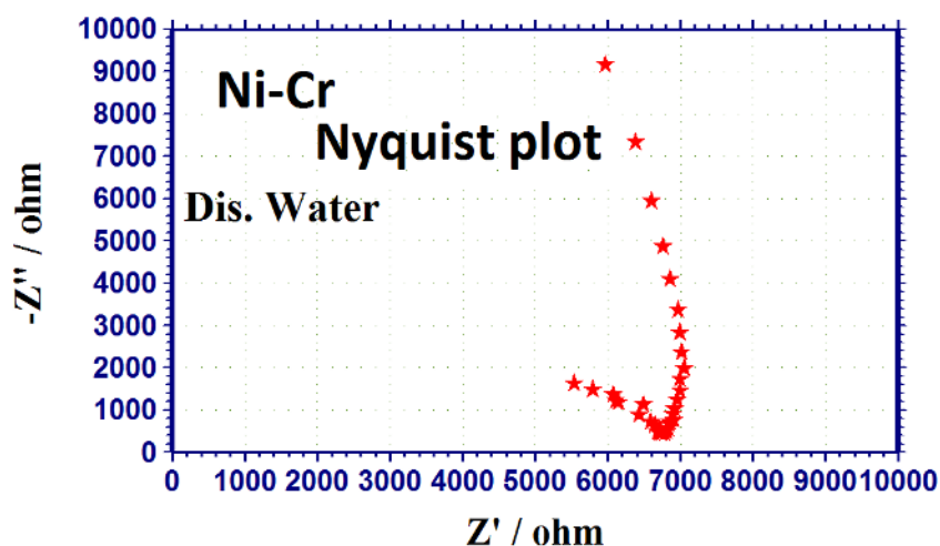
Figure 6. AC impedance spectrum of Ni–Cr immersed in distilled water (Nyquist plot).
