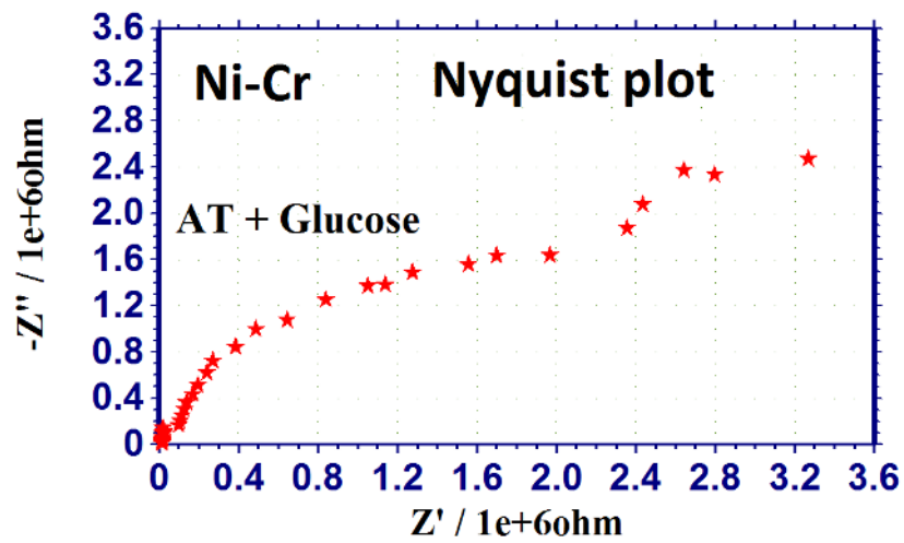
Figure 10. AC impedance spectrum of Ni–Cr immersed in artificial tears + glucose (Nyquist plot).
